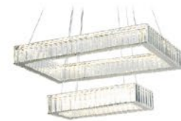
TR5005 хром 600*400*H950 LED 90W IP20 3000-6400K 46 150 p.
